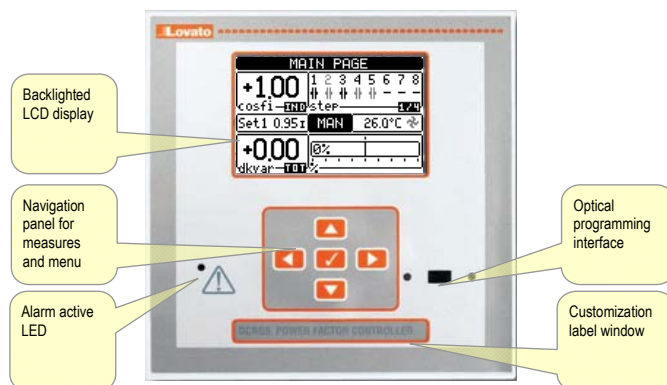
DCRG8 Front panel
